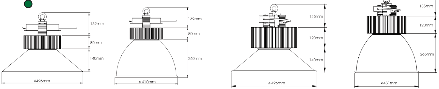
71 Degree Reflector
